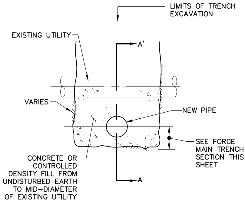
TYPICAL SECTION
