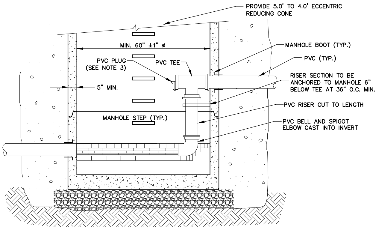
SECTION
